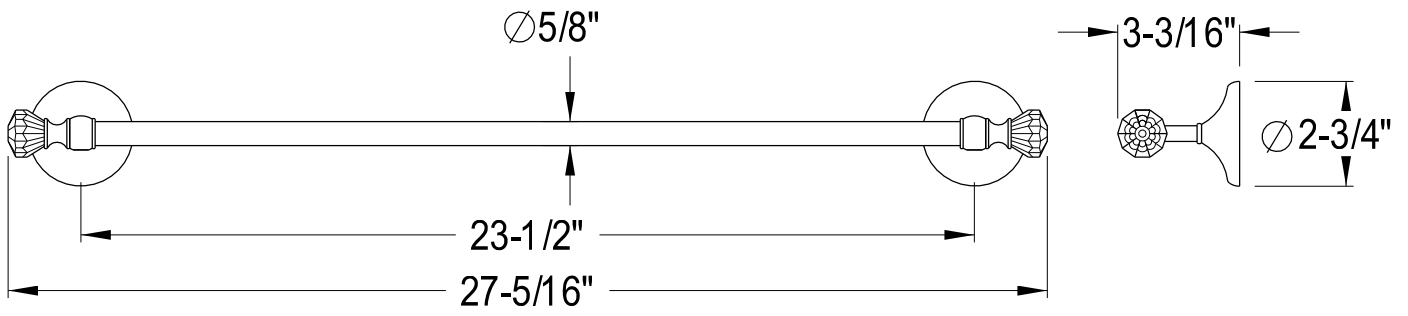
24" Towel Bar
