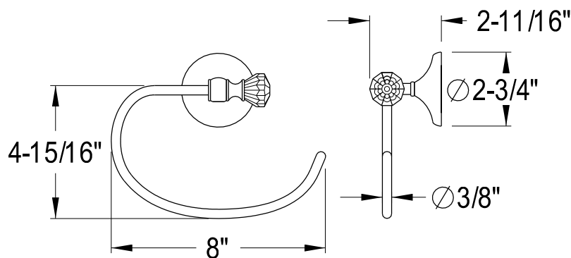
Towel Ring
