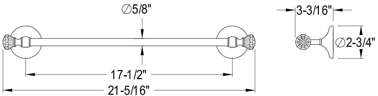
18" Towel Bar
