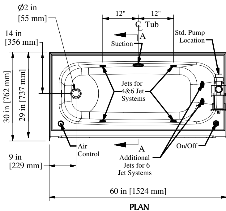
60" [1524mm] Bathtub w/ 18" [457mm] Threshold & 4 or 6 Jet Whirlpool Package
